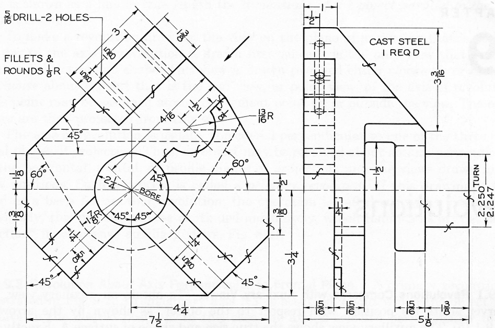
Fig. 8-57 Box Tool Holder for Turret Lathe.
