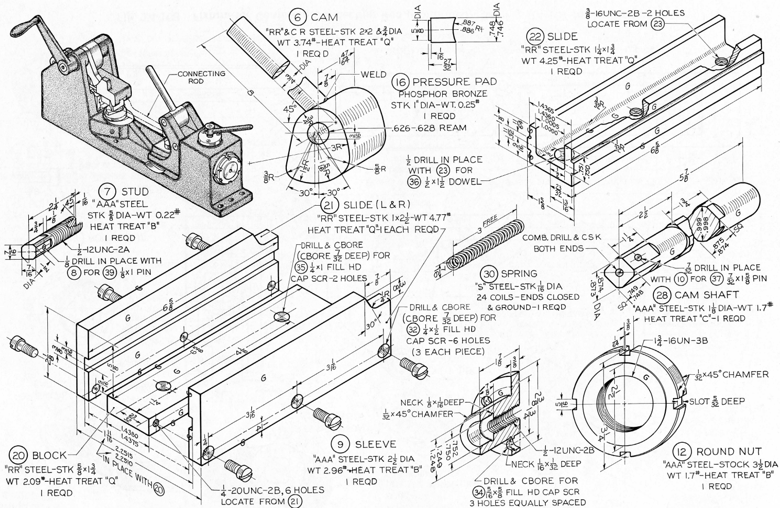
Fig. 14-107 Fixture for Centering Connecting Rod. (1) Draw details using decimal dimensions, if assigned. (2) Draw assembly. (See also Figs. 14-108 and 14-109.)
