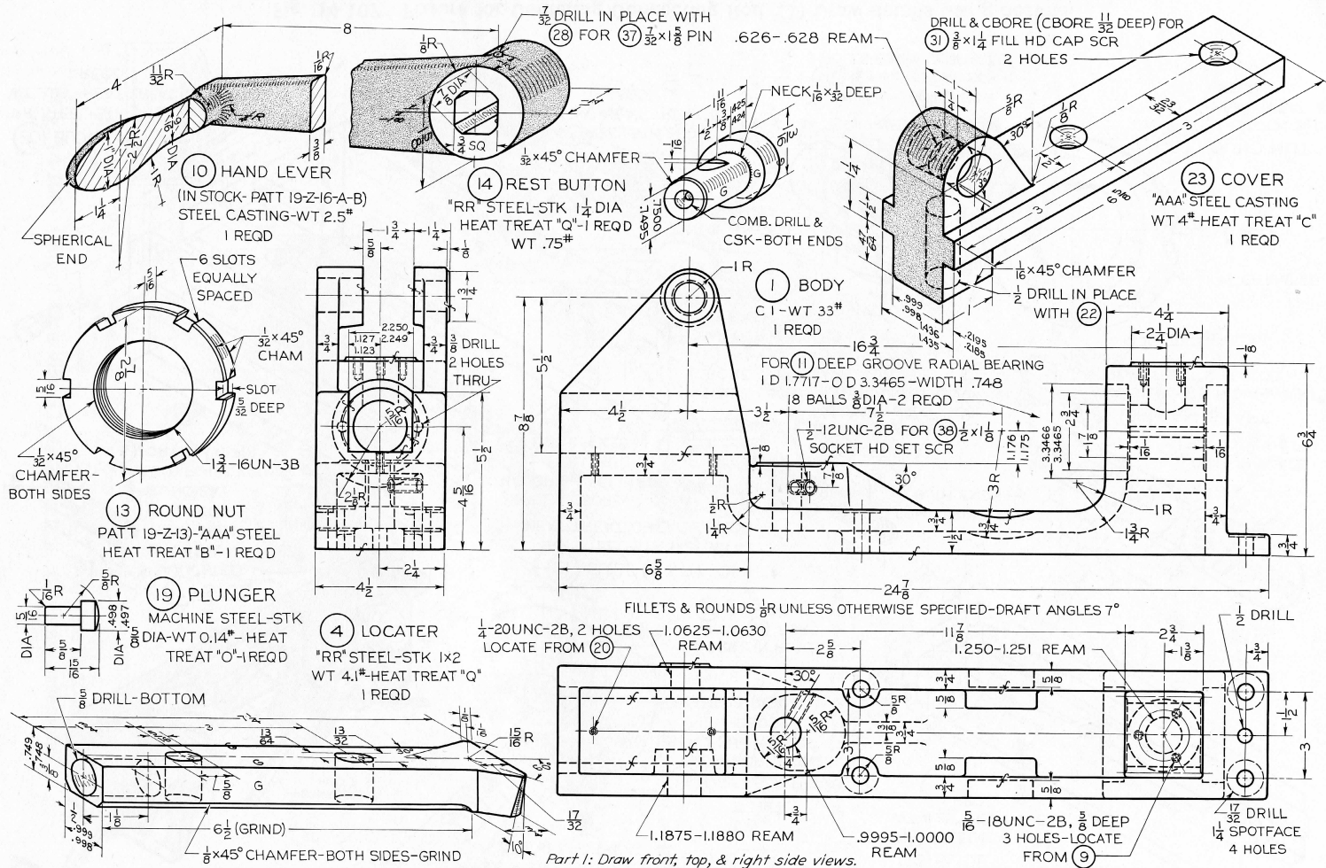
Fig. 14-108 Fixture for Centering Connecting Rod (Continued). See Fig. 14-107 for instructions.
