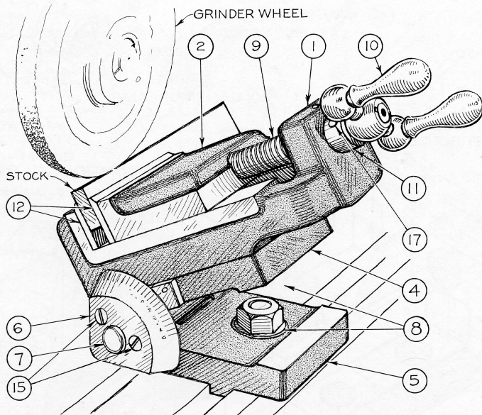
Fig. 14-74 Grinder Vise. (See Figs. 14-75 and 14-76.)
