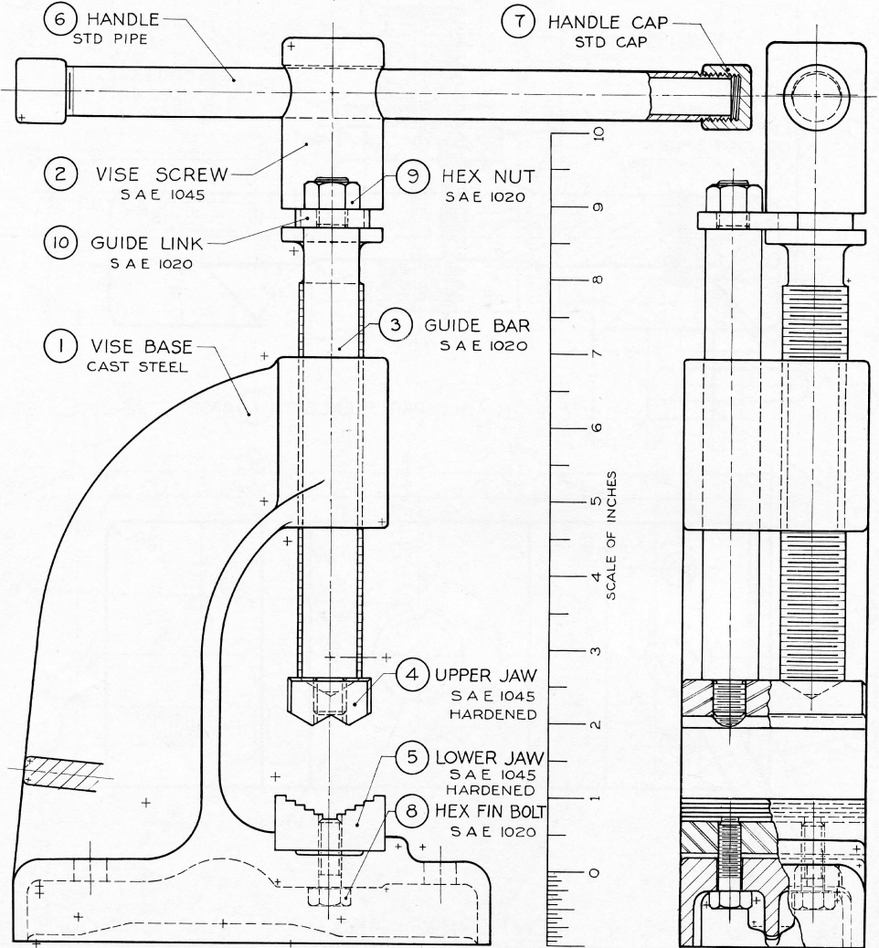
Fig. 14-68 Pipe Vise. (1) Draw details. (2) Draw assembly. To obtain dimensions, take distances directly from figure with dividers; then set dividers on printed scale and read measurements in inches. All threads are Unified and American National Coarse Threads except the American Standard Pipe Threads on Handle and Handle Caps.
