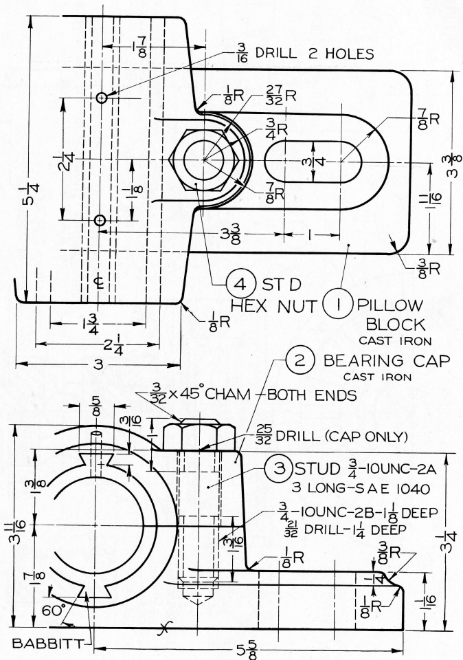
Fig. 14-66 Pillow Block Bearing. (1) Draw details. (2) Draw assembly.
