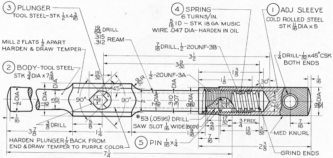
Fig. 14-62 Tap Wrench. (1) Draw details. (2) Draw assembly. If assigned, use unidirectional two-place decimals for all fractional dimensions.
