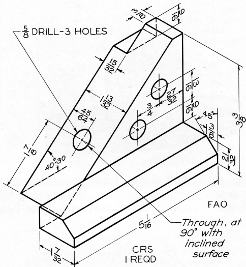
Fig. 8-43 Adjuster Block. Draw necessary views, including complete auxiliary view showing true shape of inclined surface (Layout B-4).
