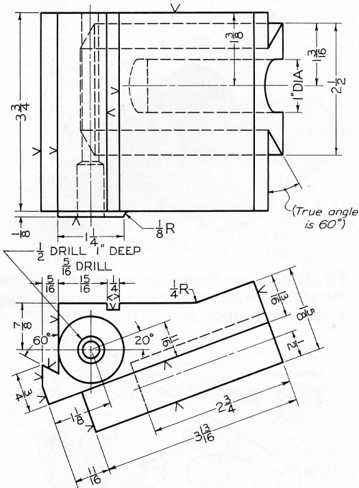
Fig. 8-42 Tool Holder Slide. Draw given views, and add complete auxiliary view showing true curvature of slot on bottom (Layout B-4).
