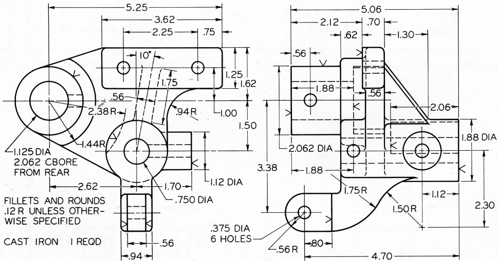
Fig. 6-119 Power Feed Bracket for Universal Grinder.
