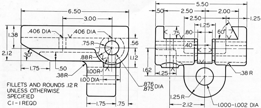
Fig. 6-118 Sliding Nut for Mortiser.
