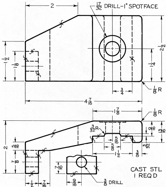
Fig. 6-114 Trip Lever.
