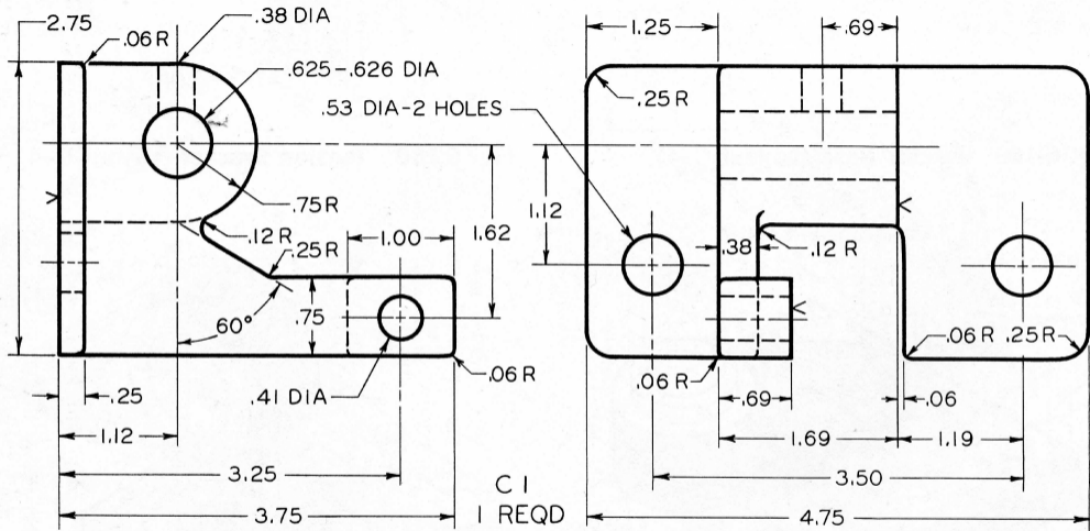
Fig. 6-115 Knurl Bracket Bearing.
