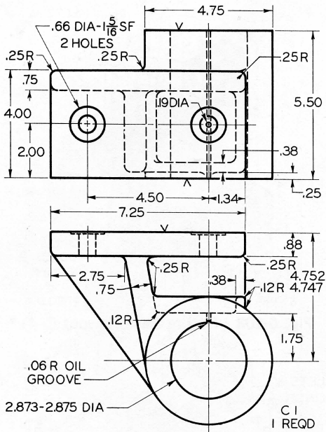
Fig. 6-113 Feed Shaft Bracket.
