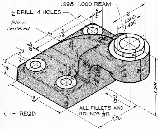
Fig. 6-111 Offset Bearing (Layout C-4).*
