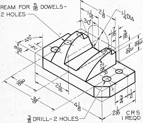
Fig. 6-65 Locating Finger (Layout A-3).*
