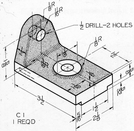
Fig. 6-67 Cut-off Holder (Layout A-3).*
