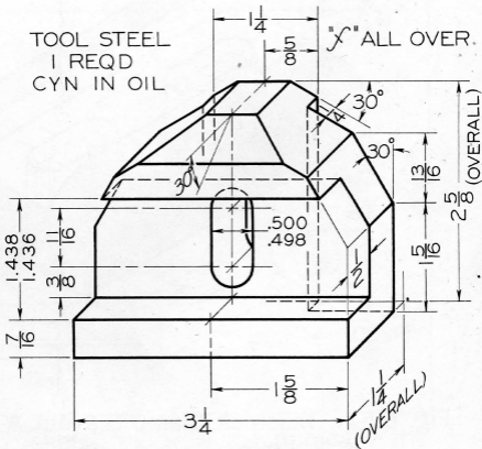
Fig. 6-64 Support (Layout A-3).*
