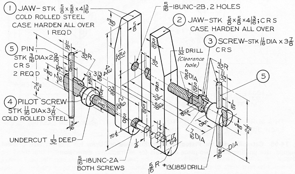
Fig. 14-57 Machinist's Clamp. Draw details and assembly. If assigned, use unidirectional two-place decimal dimensions.
