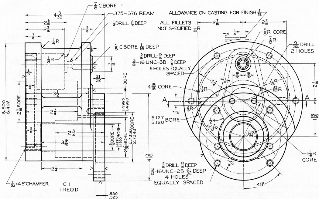
Fig. 14-53 Generator Drive Housing.
