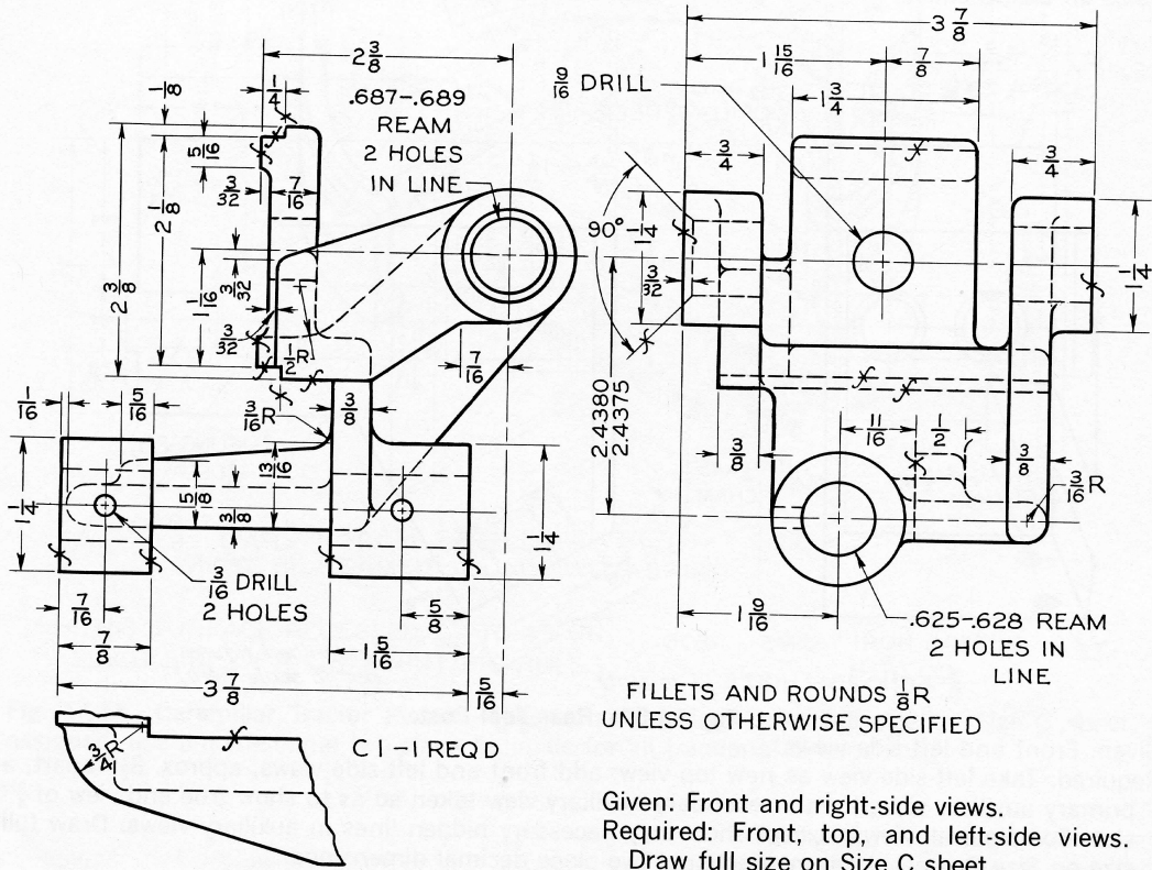
Fig. 14-52 Bearing for a Worm Gear.
