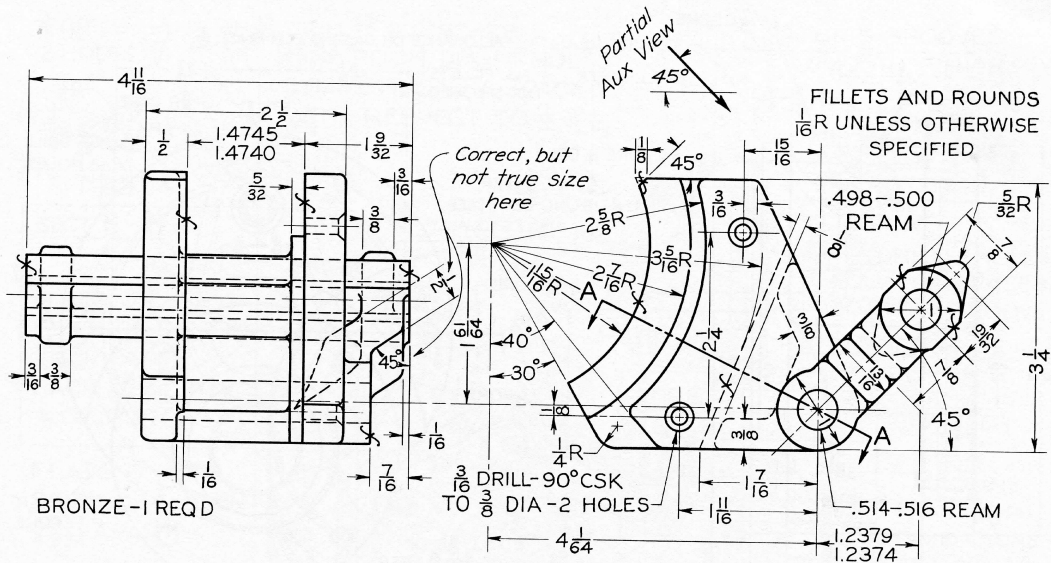
Fig. 14-51 Shifter Fork for Vertical Milling Machine.
