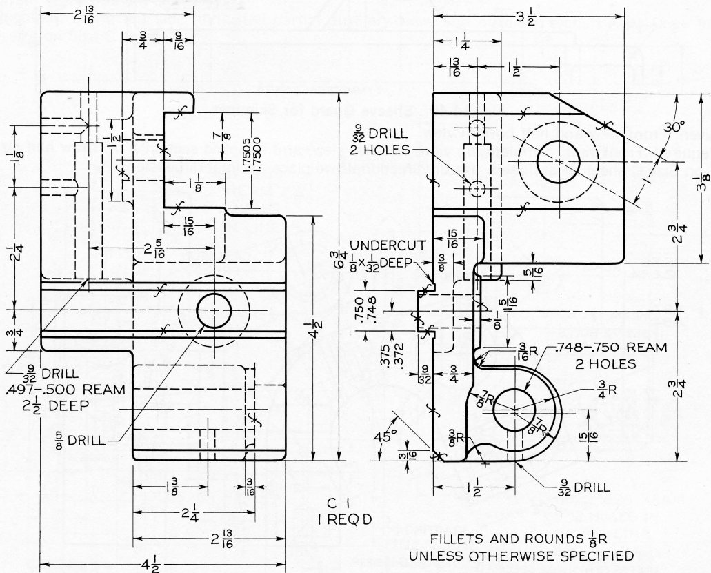
Fig. 14-48 Roller Rest Bracket for Automatic Screw Machine.
