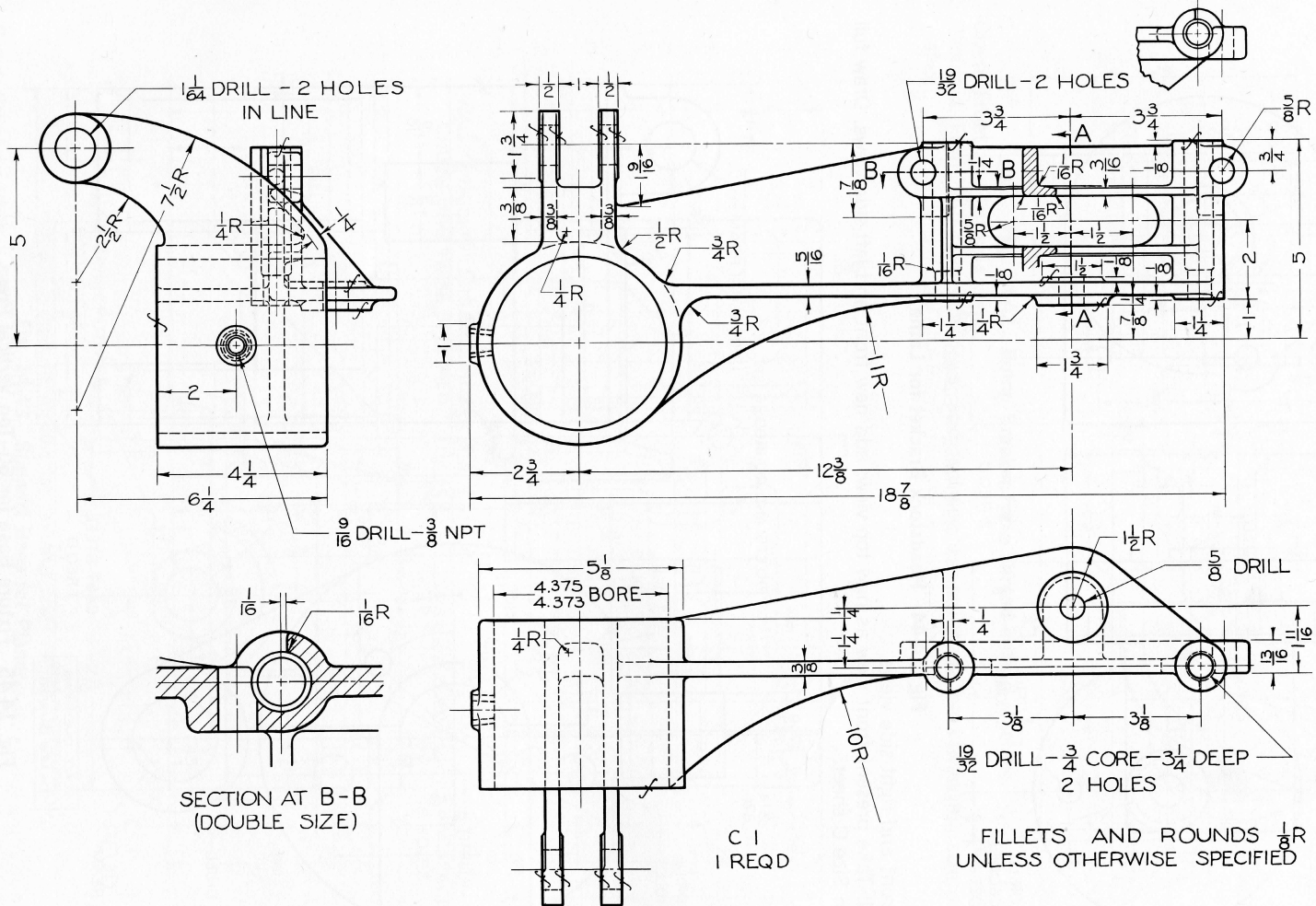
Fig. 14-46 Bracket.
