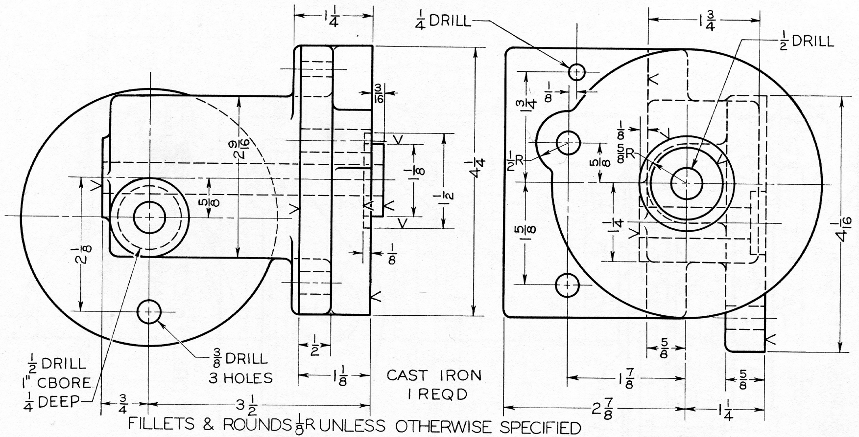
Fig. 14-44 Headstock Bracket for Lathe.
