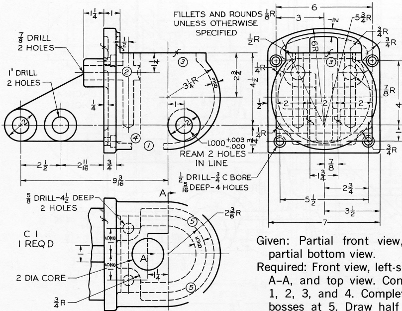
Fig. 14-41 Gear Change Lever Bracket.
