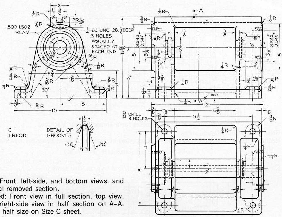
Fig. 14-40 Spindle Housing.
