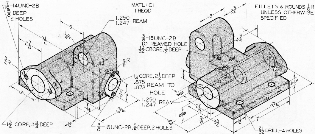
Fig. 14-38 Automatic Stop Box. Make detail drawing. Draw half size on Size B sheet.
