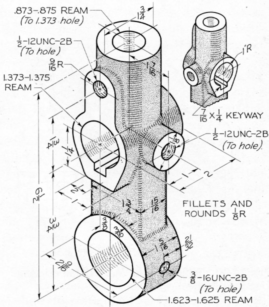
Fig. 14-34 Idler Arm. Make detail drawing. Use Size B sheet.
