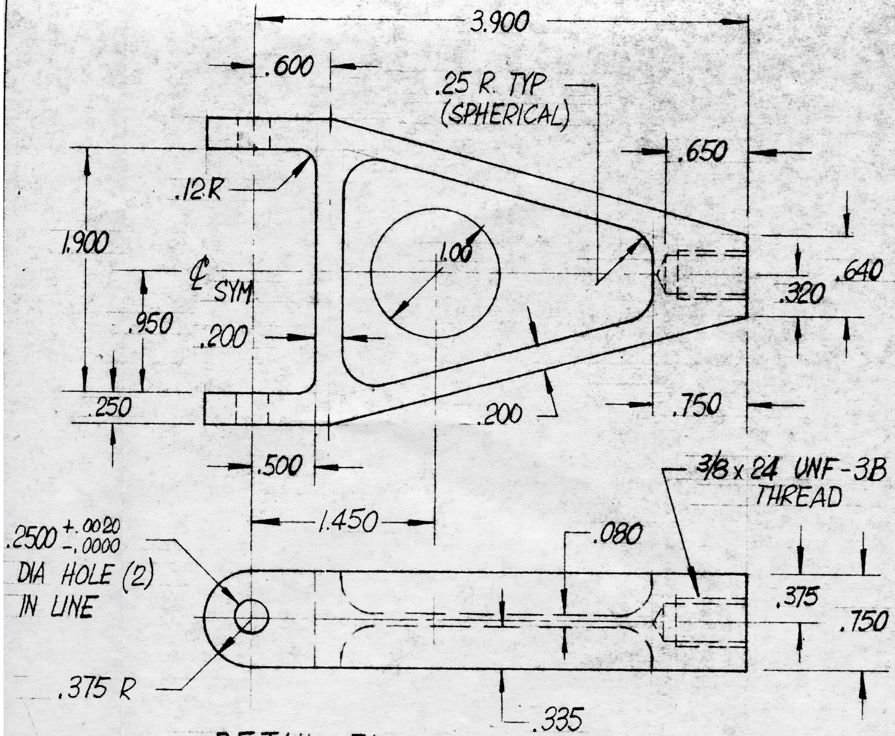
DETAIL - 71
